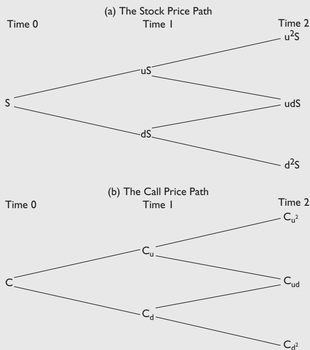
Figure 4.3 The Two-Period Binomial Tree
